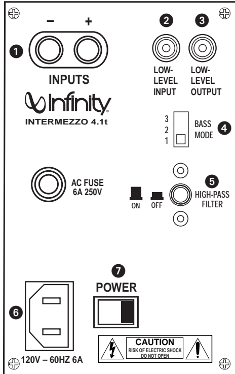
Rear Panel
