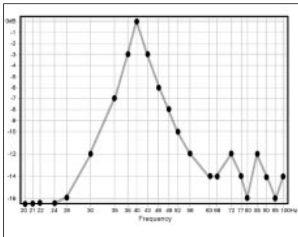
Narrow Response
