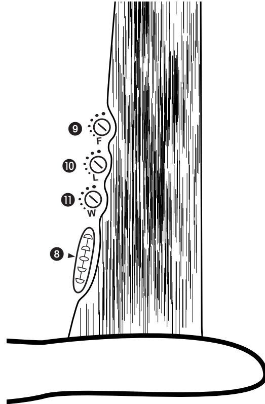
Front Panel
